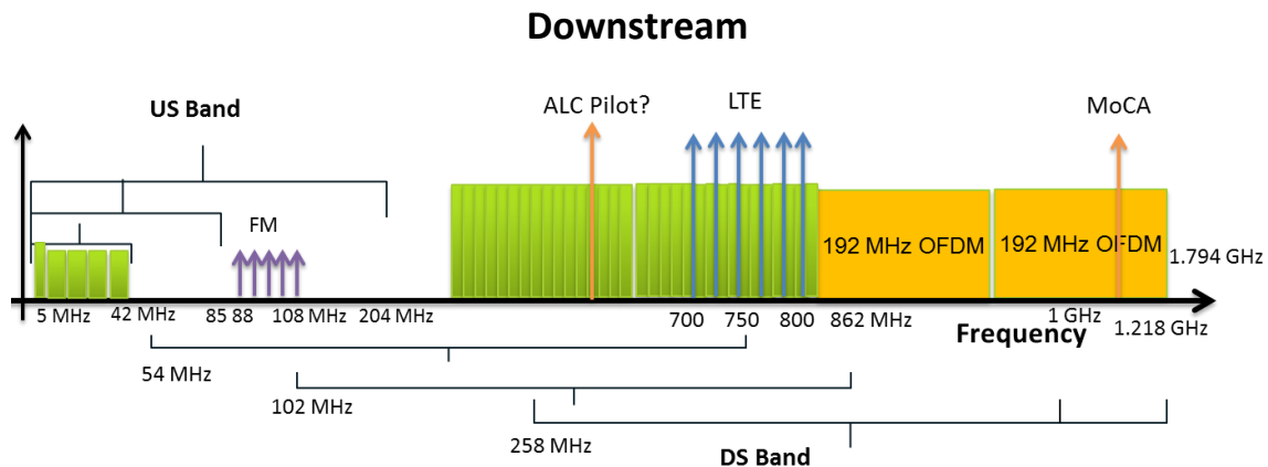
Figure 3 – D3.1 Downstream Spectrum Thoughts
