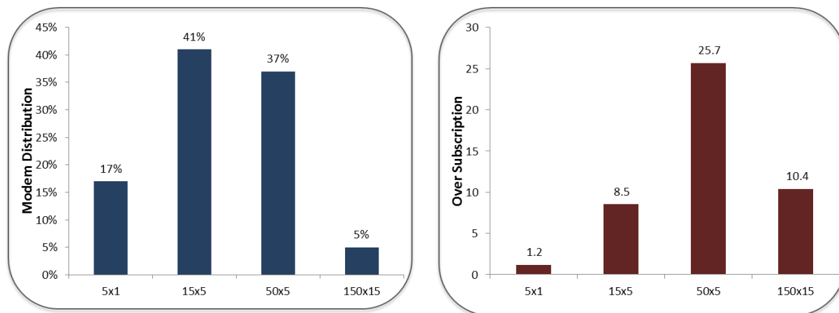
Figure 10 – Step 1 Modem Distribution and Over Subscription
