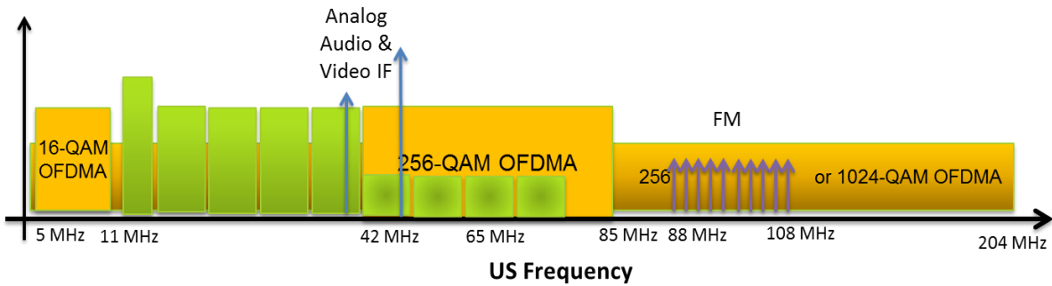
Figure 2 - Upstream Spectrum Planning
