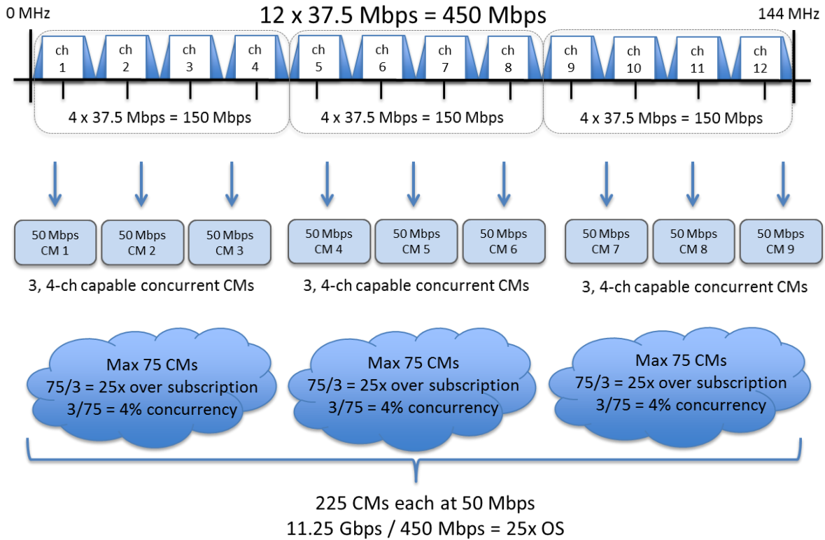
Figure 11 – 25X Over Subscription Calculation Example
