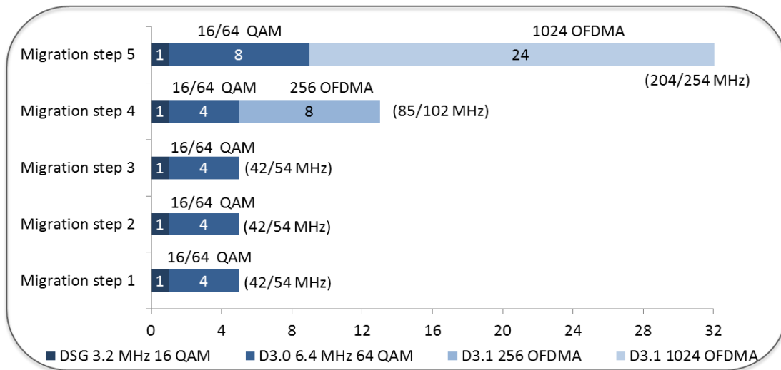
Figure 8 – US Channel Allocation
