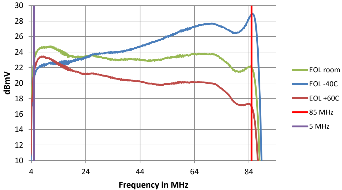
Figure 5 - US Level Swing over Temperature
