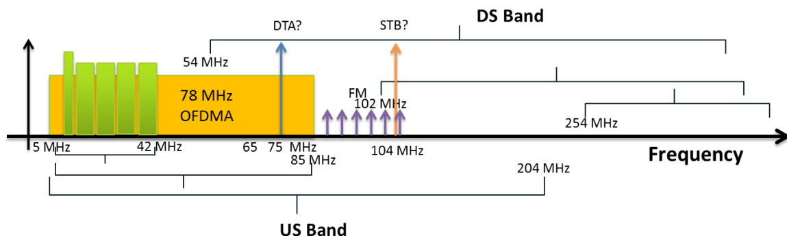
Figure 4 – D3.1 Upstream Spectrum Thoughts
