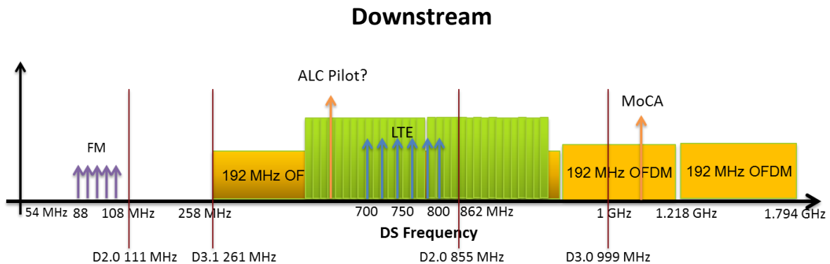
Figure 1 - Downstream Spectrum Planning
