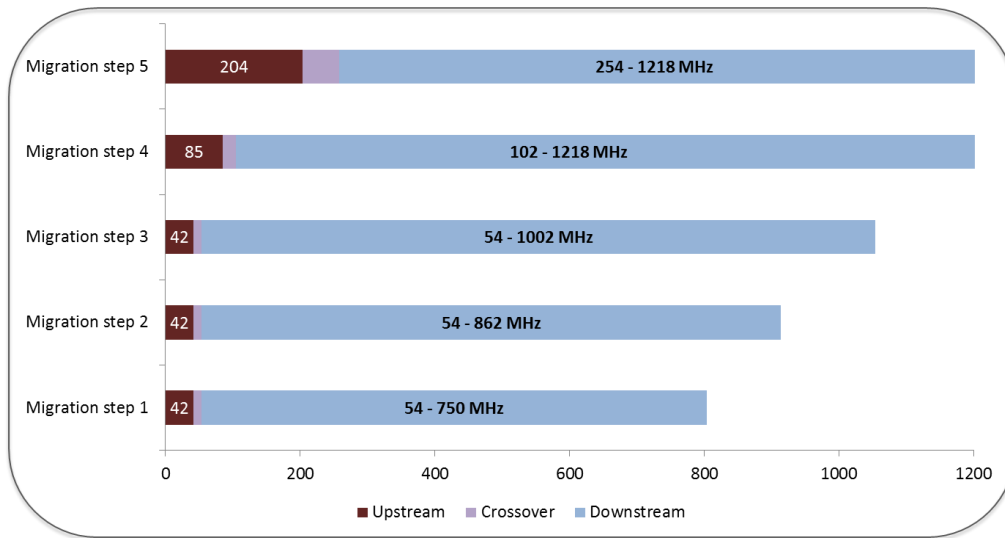
Figure 7 – DS Spectrum Allocation
