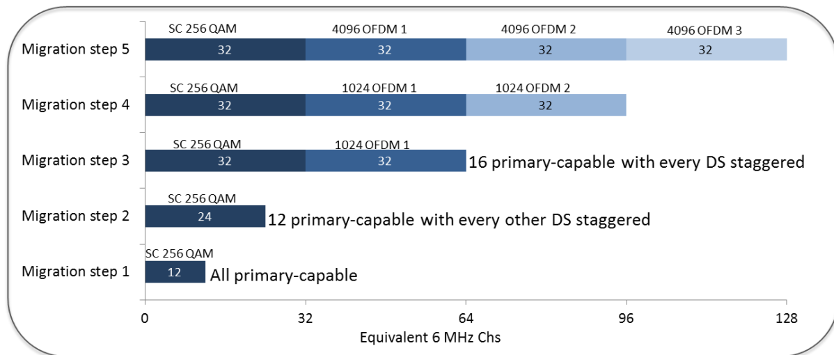
Figure 6 – DS Channel Allocation
