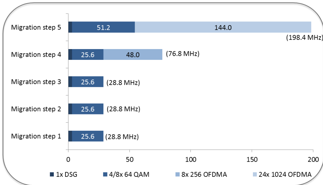
Figure 9 – US Spectrum Allocation
