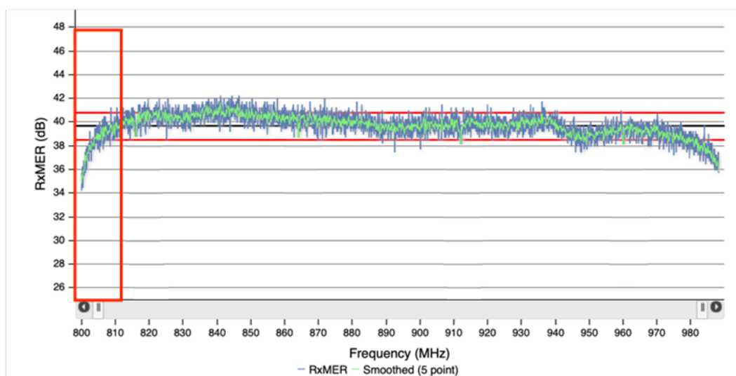
Figure 21. Another example of edge rolloff in an RxMER per subcarrier graph.
