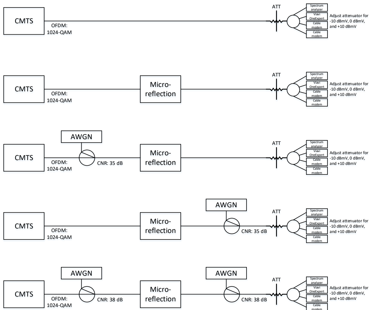
Figure 13. Equipment configurations for RxMER per subcarrier amplitude ripple testing.
