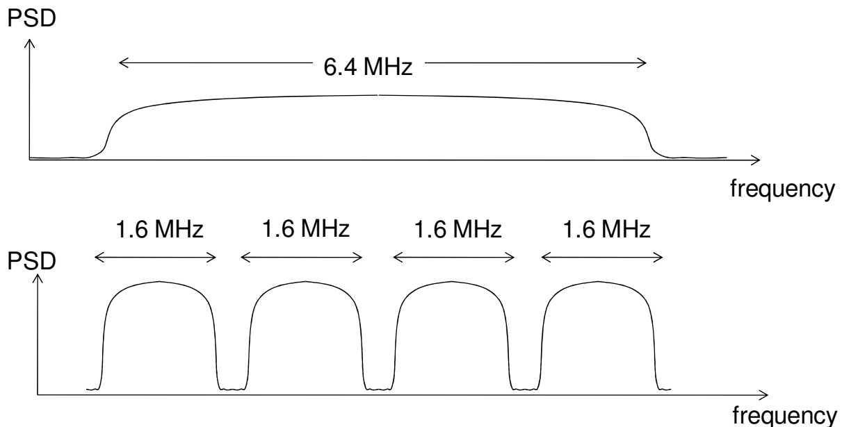
Fig. 9- Single Wide Channel vs. Four Narrow Channels (Channel Bonded)
