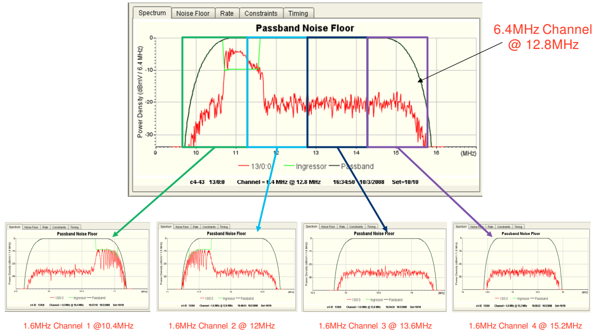
Fig. 11- Power Spectral Density of Semi-AWGN Sample
